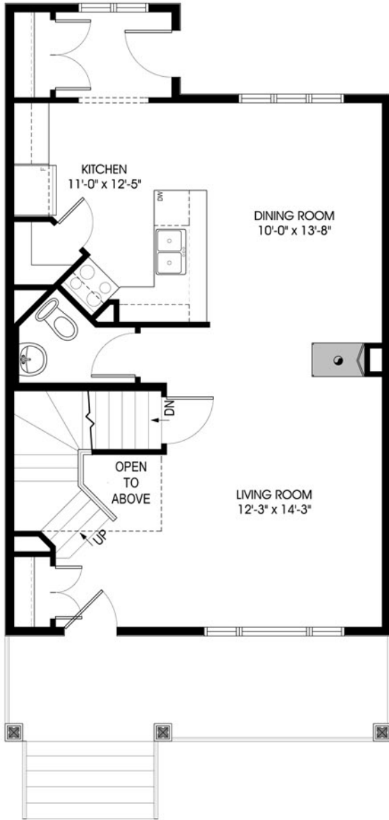
MAIN FLOOR PLAN 730 sq.ft.
